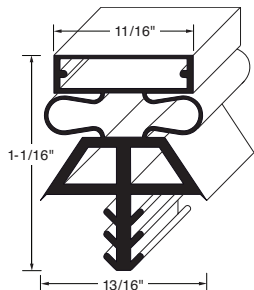
Profile MD30 Order No. 90-1032
