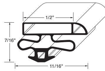
Profile MD41 Order No. 90-1040
