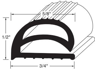
Profile CS1 Order No. 90-1000
