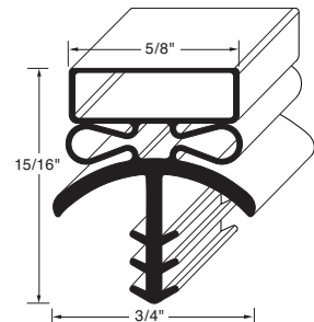
Profile MD28 Order No. 90-1031
