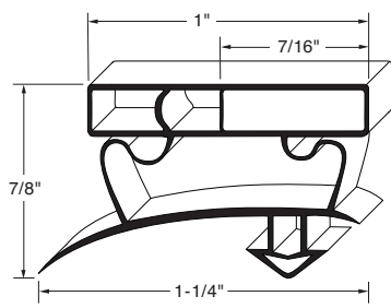
Profile MD39 Order No. 90-1033
