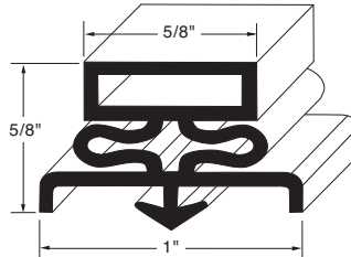
Profile MD6 Order No. 90-1005
