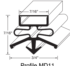
Profile MD11 Order No. 90-1028 (Black) or 90-1043 (Gray)
