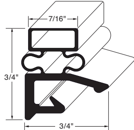
Profile MS8 Order No. 90-1035
