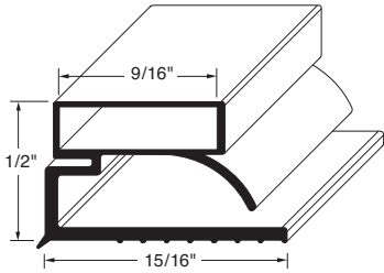
Profile MS5 Order No. 90-1003
