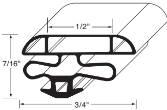
Profile MD8 Order No. 90-1026
